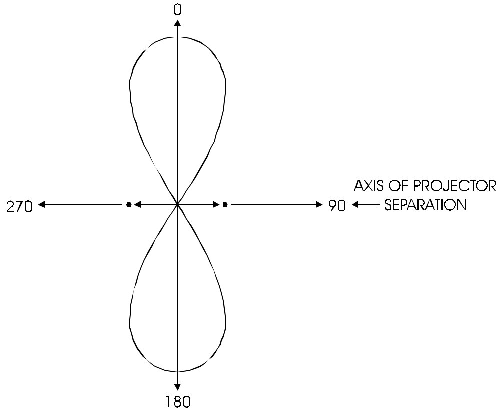
Figure Chapter 3 - -6: Beam Pattern for Two Hydrophones with Spacing l/2
