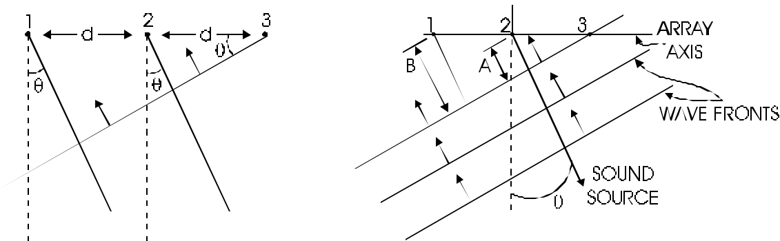
Figure Chapter 3 - -16: Wavefronts Striking a Hydrophone Array from a Source at Angle q
