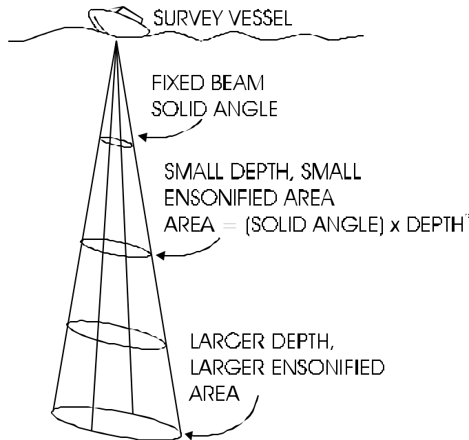
Figure Chapter 2 - -8: Dependence of Ensonified Area on Depth
