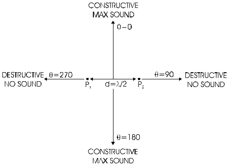
Figure Chapter 3 - -5: Directions of Constructive and Destructive Interference for Two Projectors with Spacing 1/2
