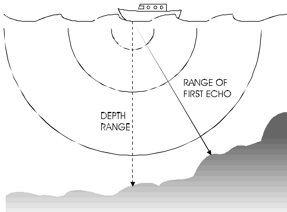
Figure Chapter 2 - -5: Surveying an Irregular Sea Floor
