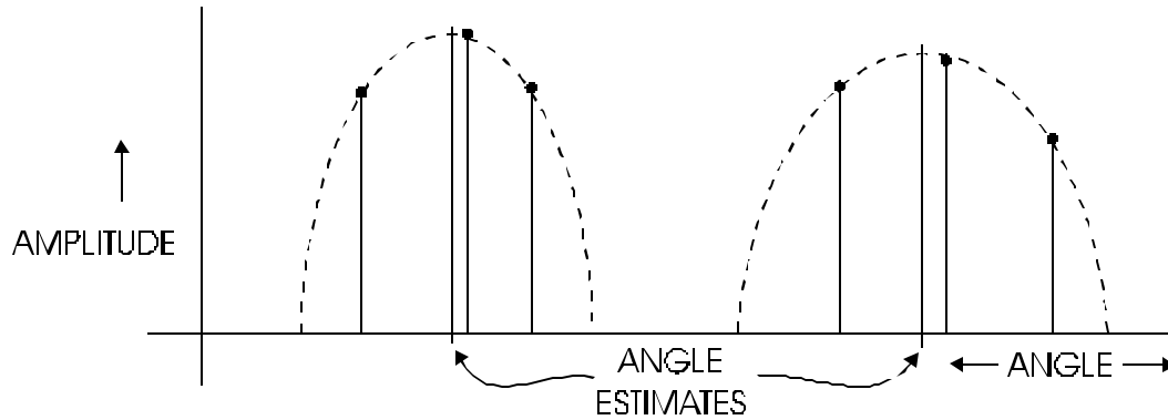
Figure Chapter 4 - -11: Parabola Fitting for High-Resolution Angle Estimation
